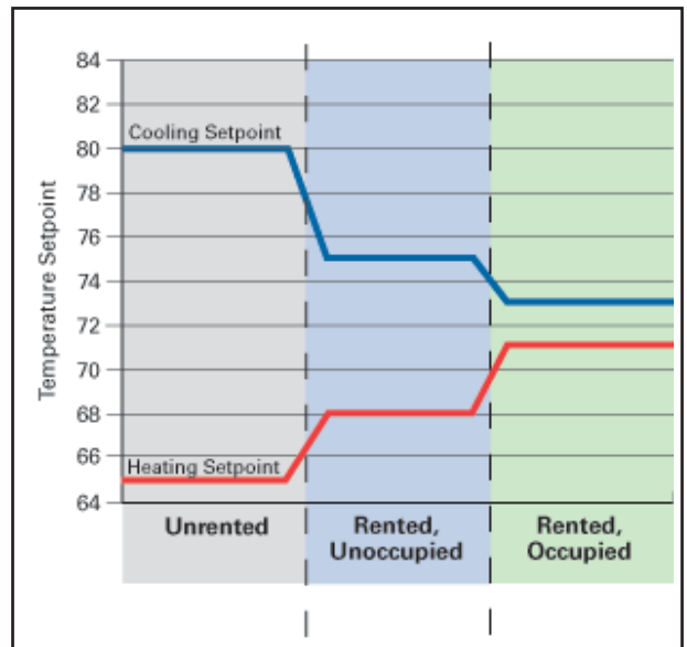
Three Modes of Guest Room FCU Operation
